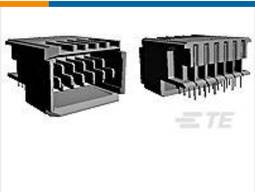
TE Part # 5-5223974-1 UPM PIN ASSY, HI CURRENT
